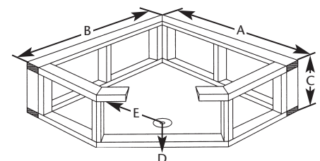
Framing – Corner Bathtub
