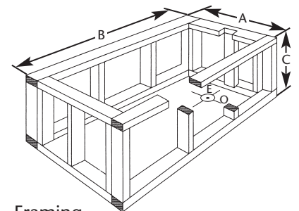
Framing Rectangular Bathtub
